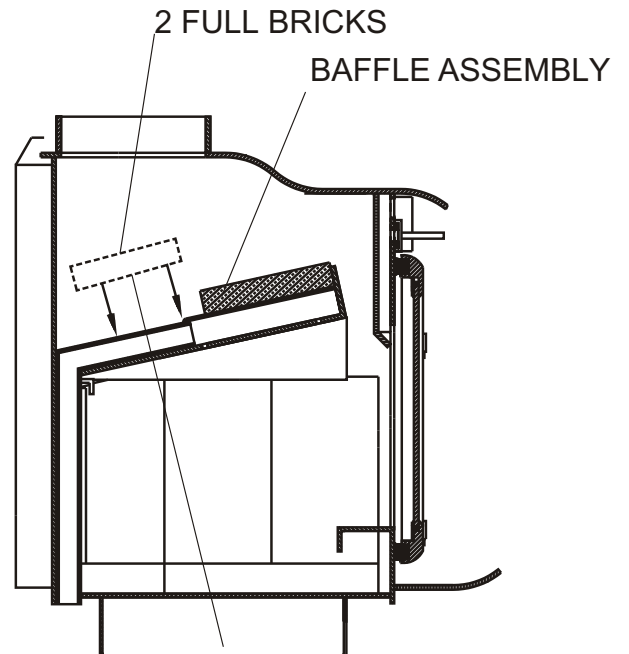
BAFFLE BRICK INSTALLATION CJW 1000 AND CJW 1500 SERIES
